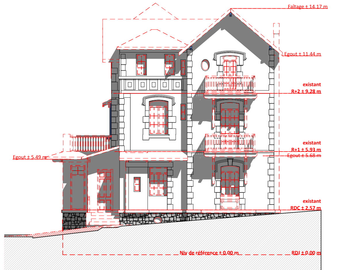
FACADE SUD - DEMOLITION
