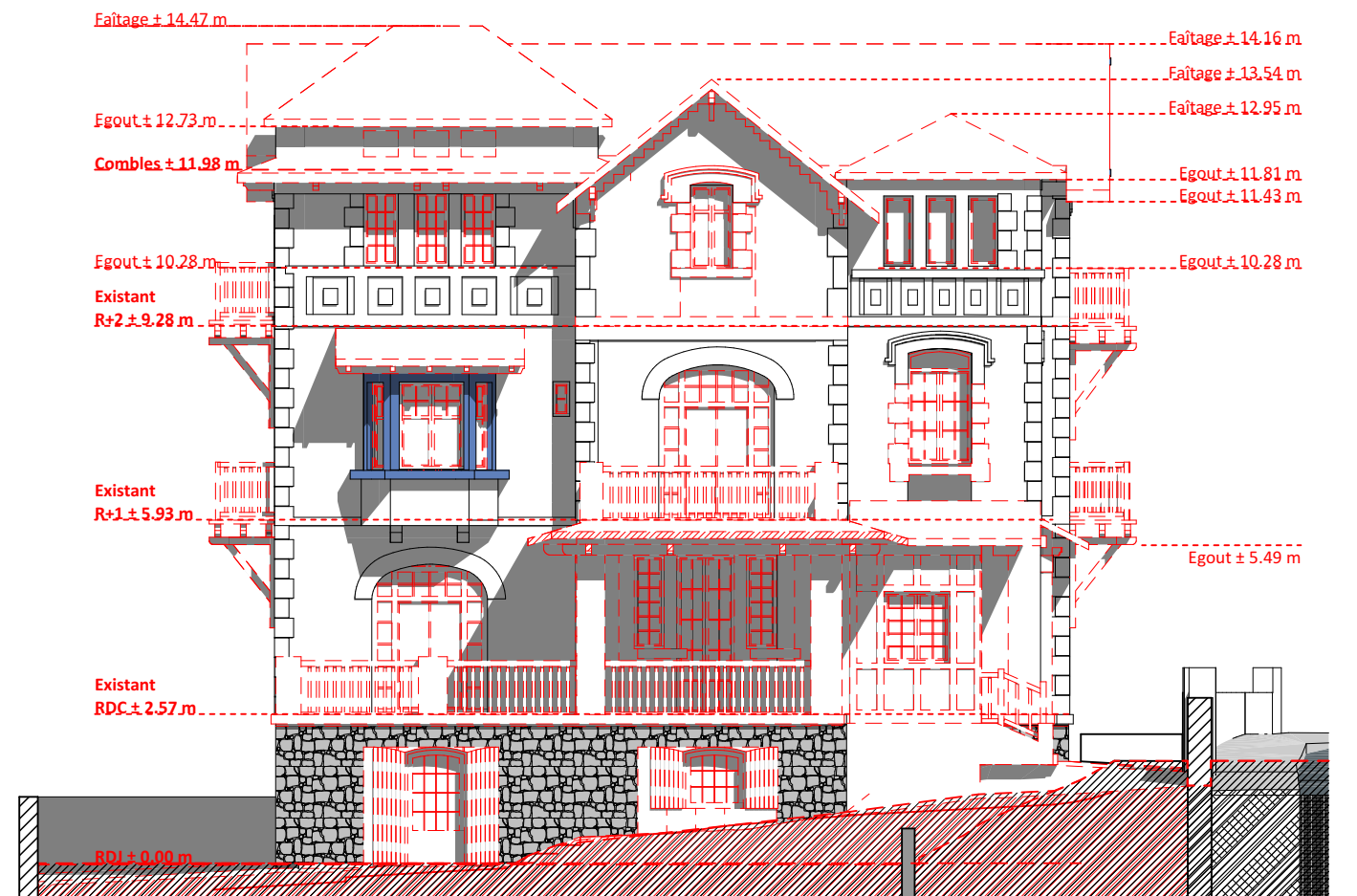
FACADE OUEST - DEMOLITION
