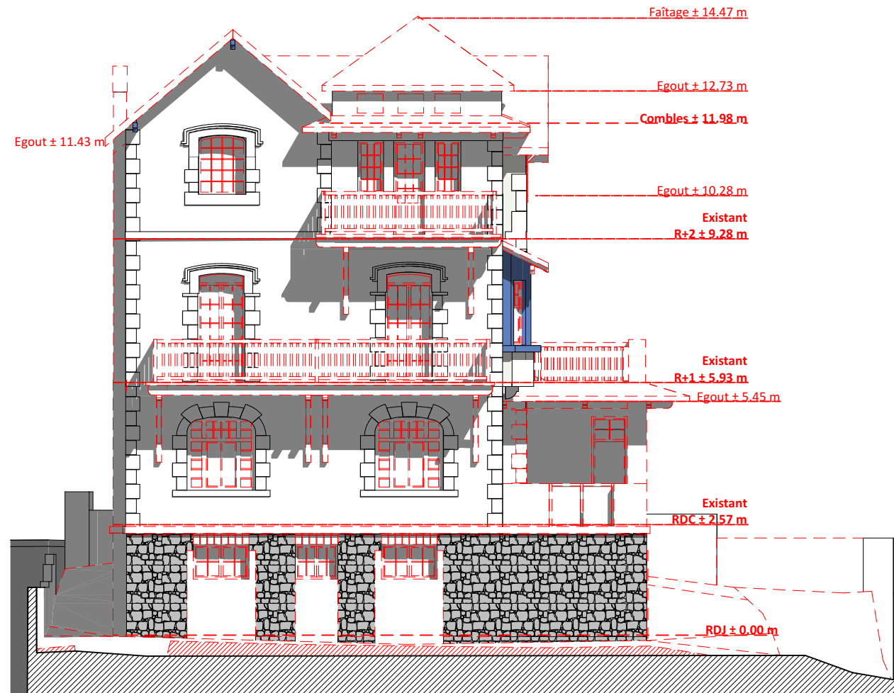
FACADE NORD - DEMOLITION
